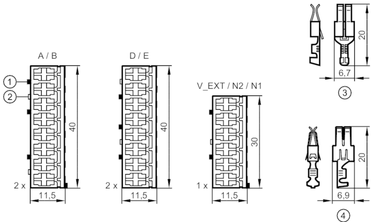
Figure shows contact housing with closed covers View on contact plug-in side
