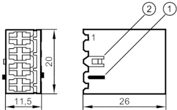
Figure shows contact housing with closed cover View on contact plug-in side
